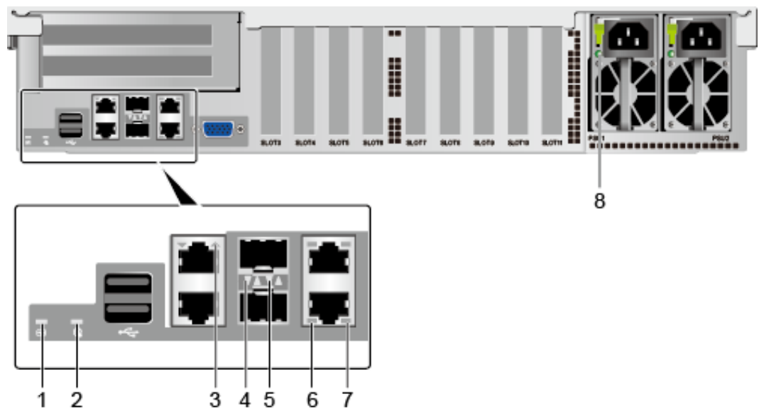
Figure 4-14 Indicators on the rear panel
