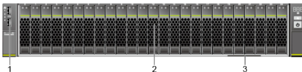
Figure 4-7 Front panel of a server with 25 SAS/SATA drives
