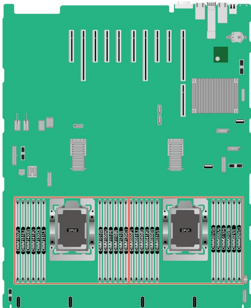
Figure 6-1 DIMM slots
